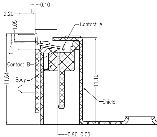
SECT:A-A
