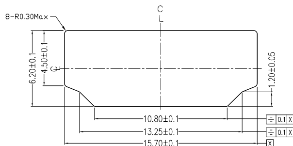
REFERENCE PANEL CUT OUT DIMENSION
