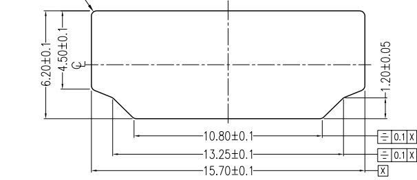
REFERENCE PANEL CUT OUT DIMENSION
