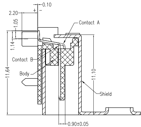
SECT:A-A
